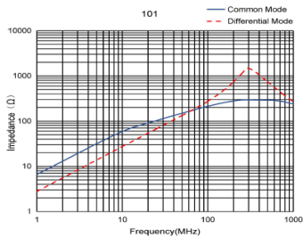
Impedance vs Frequency Curve
